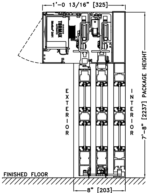
① VERTICAL SECTION WITHOUT TRANSOM
