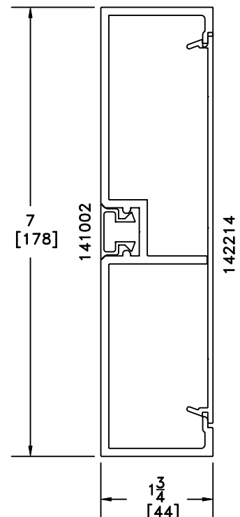
142210 1 3/4" X 7" CONCEALED FASTENER TUBE
