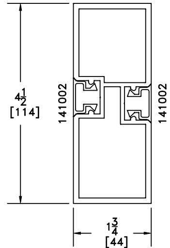
141011 1 3/4" X 4 1/2" CONCEALED FASTENER TUBE
