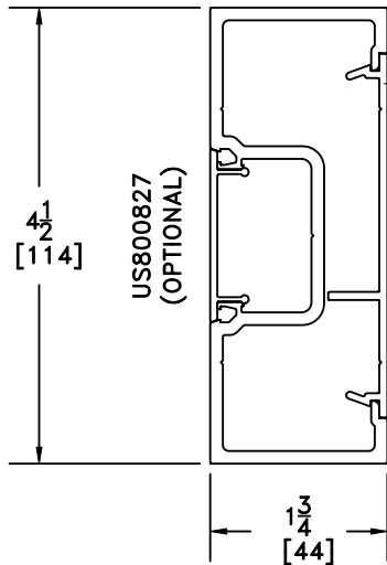
US800956 1 3/4" X 4 1/2" POCKET GLAZED "PG" TUBE
