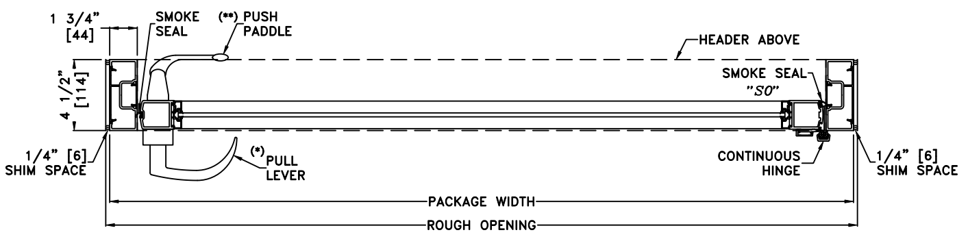
2 HORIZONTAL SECTION
