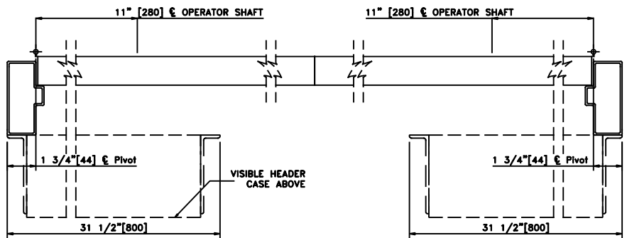
① HORIZONTAL SECTION
