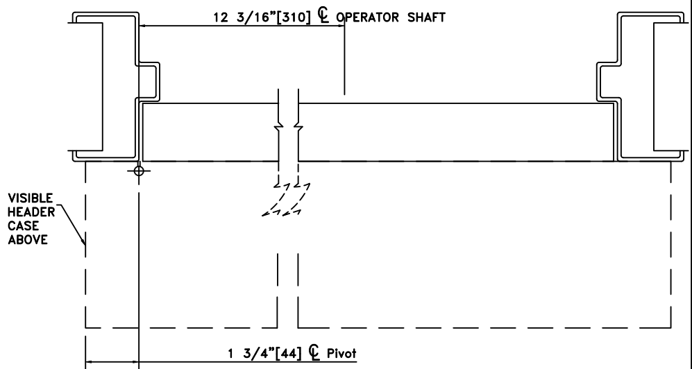
2 HORIZONTAL SECTION
