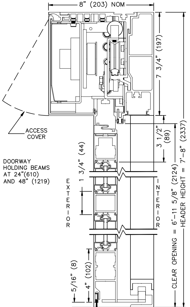
VERTICAL SECTION (NOT TO SCALE)
