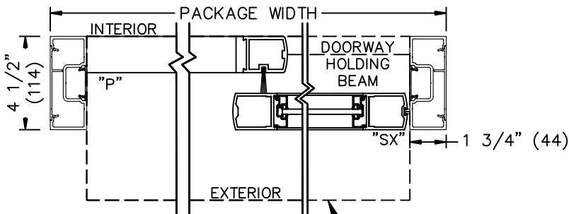
HORIZONTAL SECTION
