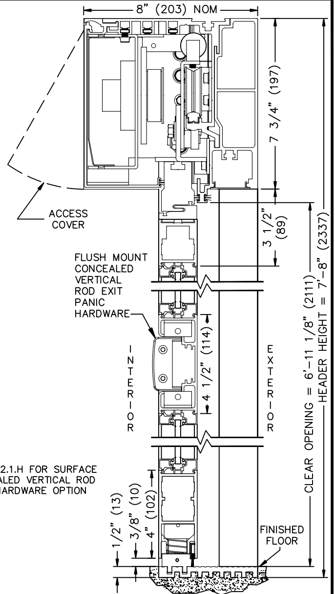
① VERTICAL SECTION (NOT TO SCALE)
