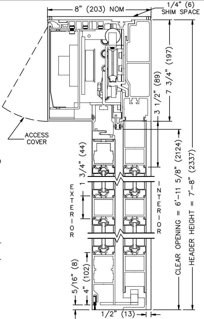
VERTICAL SECTION (NOT TO SCALE)
