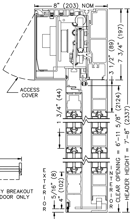
① VERTICAL SECTION (NOT TO SCALE)
