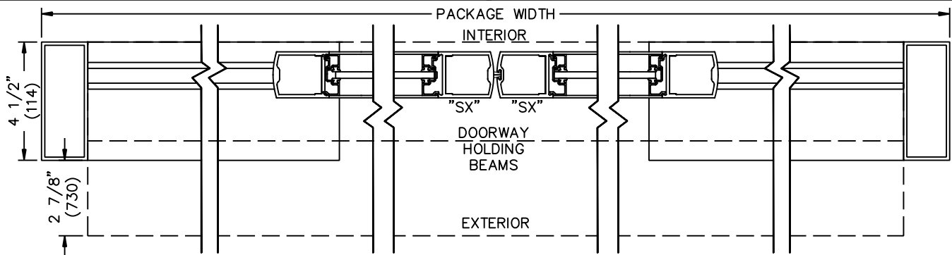
② HORIZONTAL SECTION - BI-PART SLIDER
