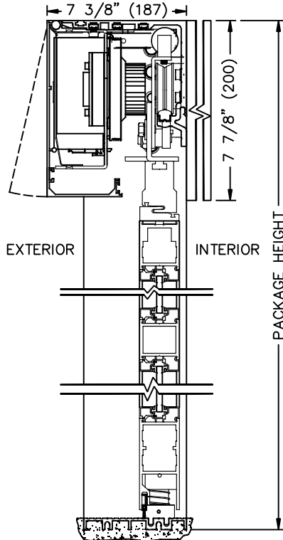
① VERTICAL SECTION WITHOUT TRANSOM
