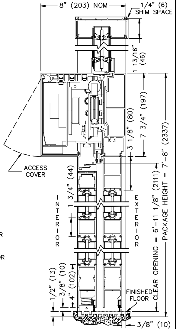
① VERTICAL SECTION (NOT TO SCALE)
