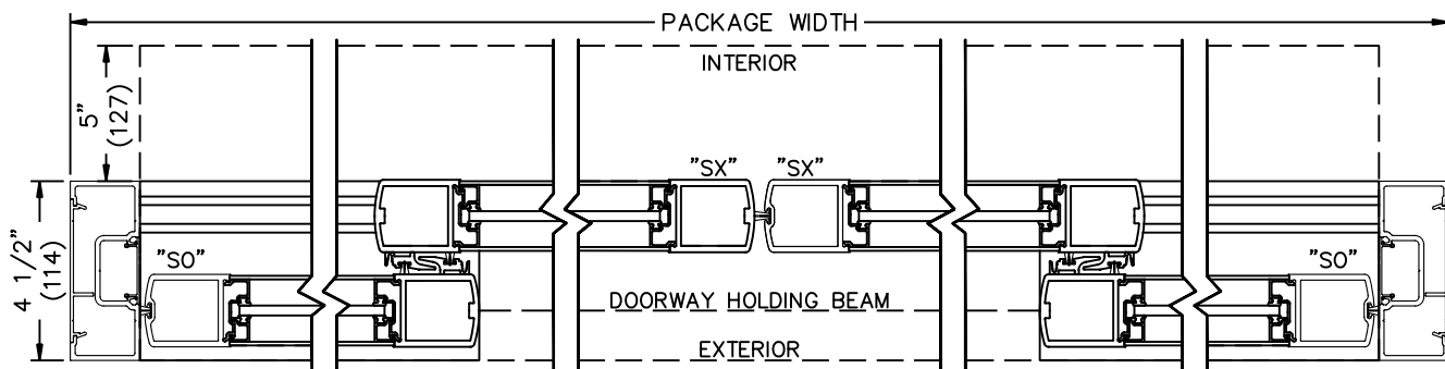
② HORIZONTAL SECTION - BI-PART SLIDER
