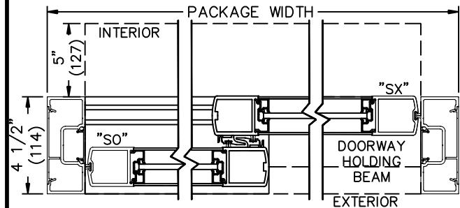
② HORIZONTAL SECTION - L.H. SINGLE SLIDE
