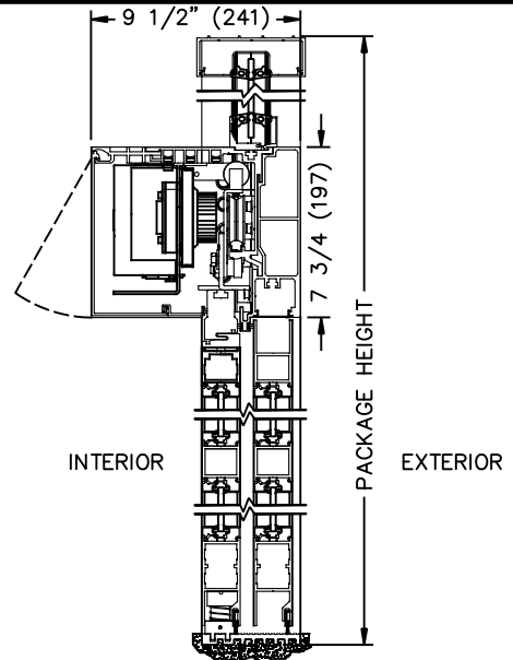
① VERTICAL SECTION WITH TRANSOM
