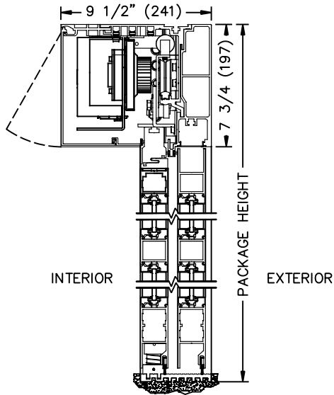
① VERTICAL SECTION WITHOUT TRANSOM
