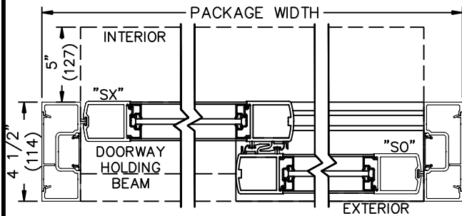
② HORIZONTAL SECTION - R.H. SINGLE SLIDE
