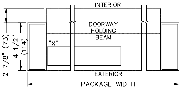
② HORIZONTAL SECTION – R.H. SINGLE SLIDE
