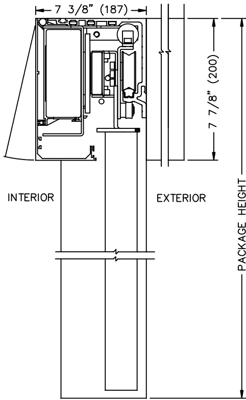
① VERTICAL SECTION WITHOUT TRANSOM
