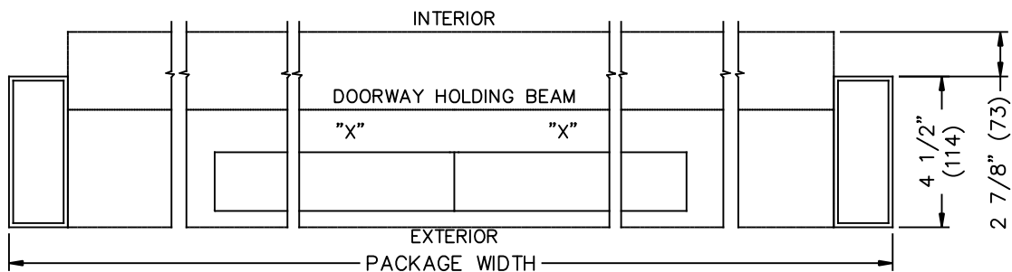
② HORIZONTAL SECTION – BI-PART SLIDER
