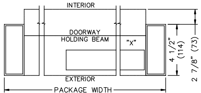
② HORIZONTAL SECTION – L.H. SINGLE SLIDE
