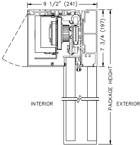
① VERTICAL SECTION WITHOUT TRANSOM
