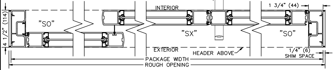
② HORIZONTAL SECTION
