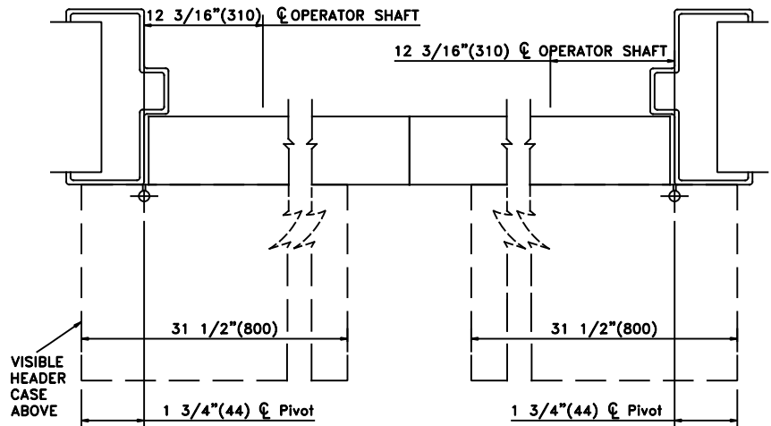
2 HORIZONTAL SECTION
