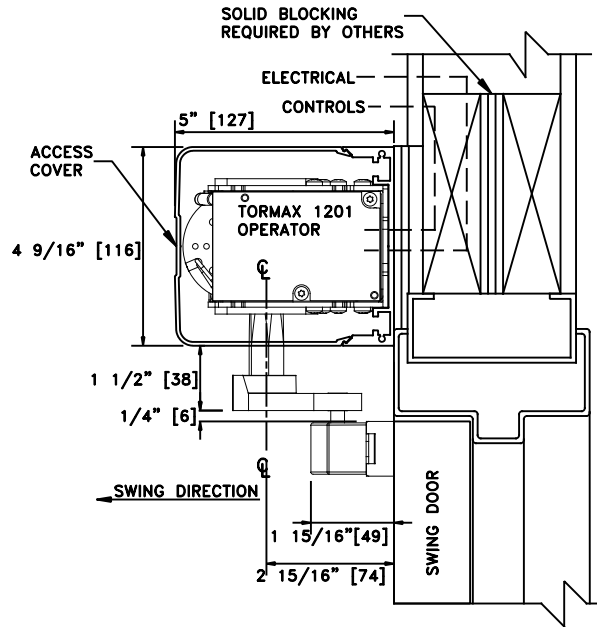
1 VERTICAL SECTION
