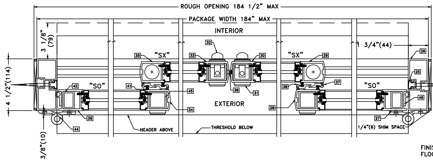
HORIZONTAL SECTION
