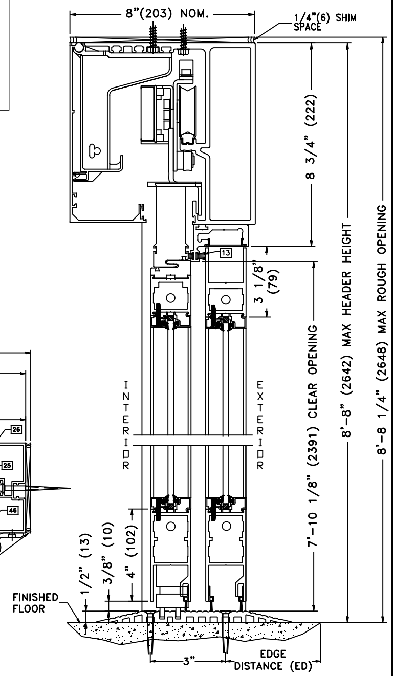
VERTICAL SECTION
