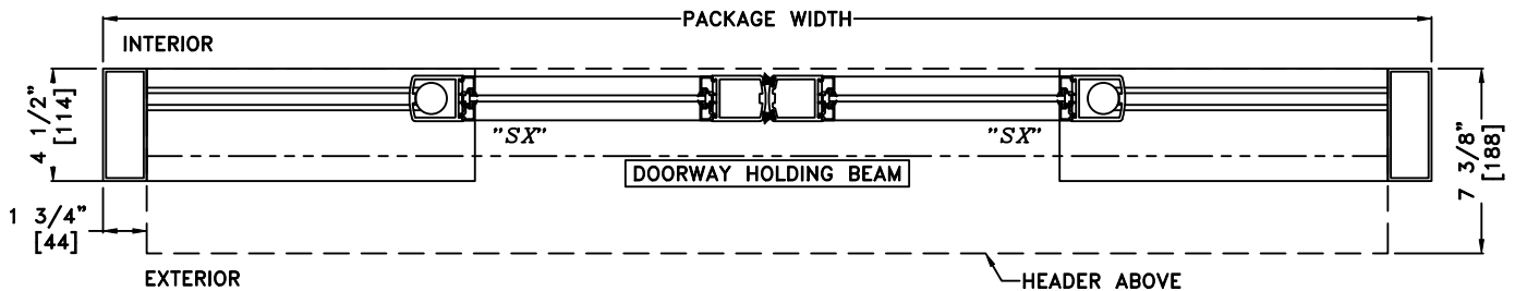
② HORIZONTAL SECTION - BIPART SLIDER
