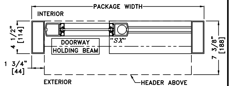
② HORIZONTAL SECTION - RH SINGLE SLIDE
