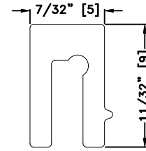
THRESHOLD TRACK GROOVE FILLER STRIP - RUNS THROUGH SLIDE DOOR OPENING ON ALL SLIDE DOOR TRACKS
