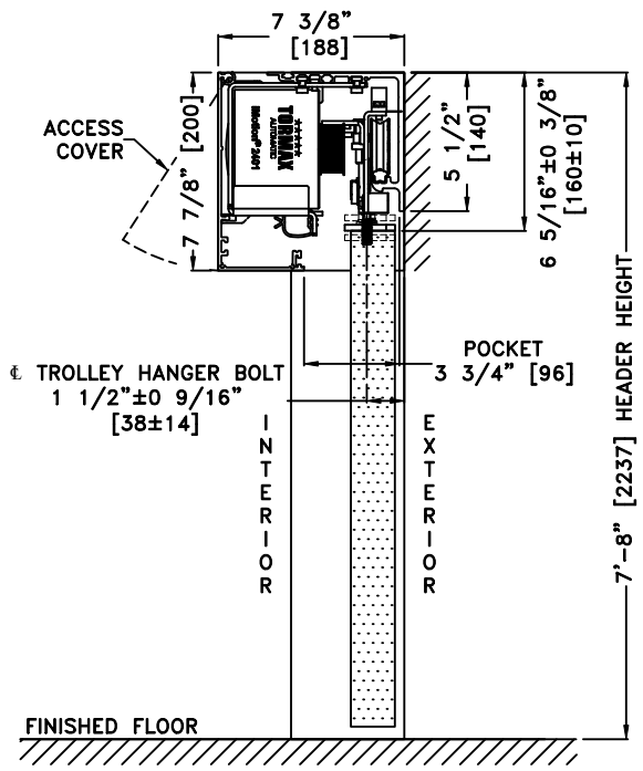
① VERTICAL SECTION WITHOUT TRANSOM
