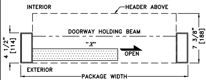
② HORIZONTAL SECTION - RH SINGLE SLIDE
