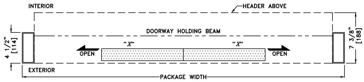
② HORIZONTAL SECTION - BIPART SLIDER
