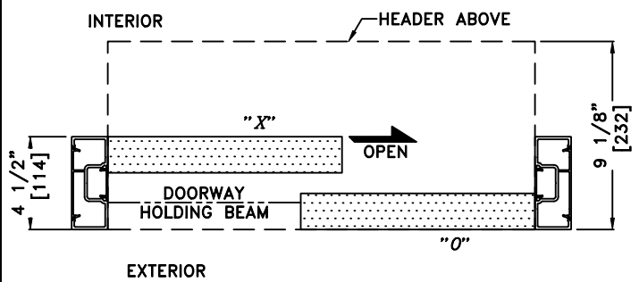
② HORIZONTAL SECTION - RH SINGLE SLIDE
