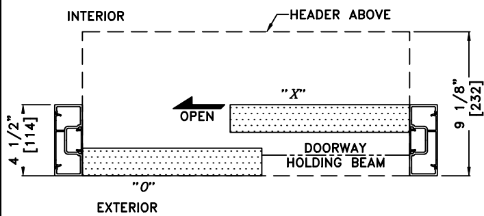
② HORIZONTAL SECTION - LH SINGLE SLIDE
