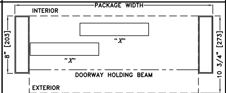
② HORIZONTAL SECTION - RH SINGLE SLIDE
