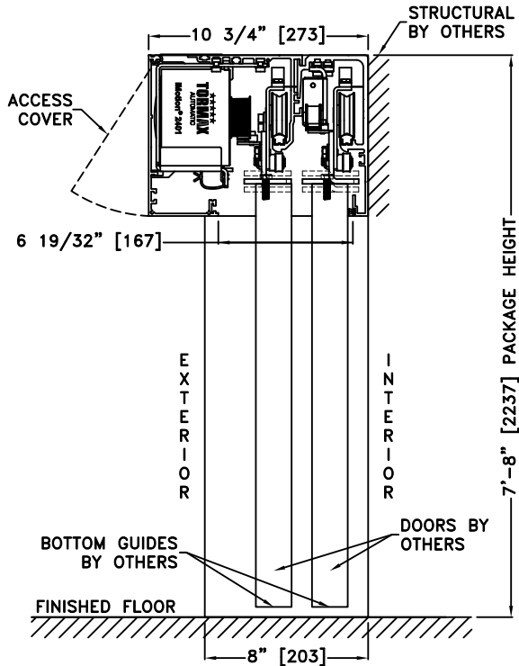
① VERTICAL SECTION WITHOUT TRANSOM
