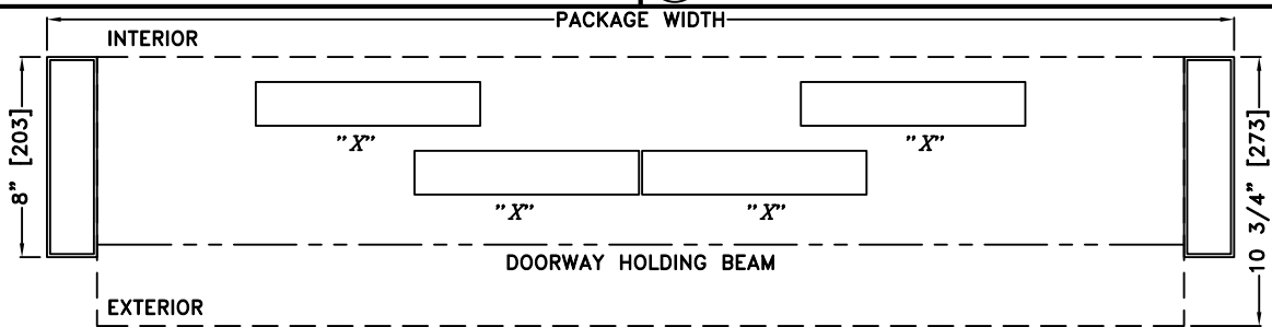
② HORIZONTAL SECTION - LH SINGLE SLIDE
