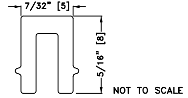
THRESHOLD TRACK GROOVE FILLER STRIP – RUNS FULL WIDTH ON ALL THRESHOLDS
