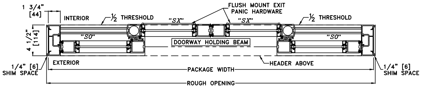
2 HORIZONTAL SECTION
