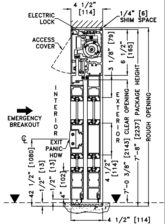
1 VERTICAL SECTION
