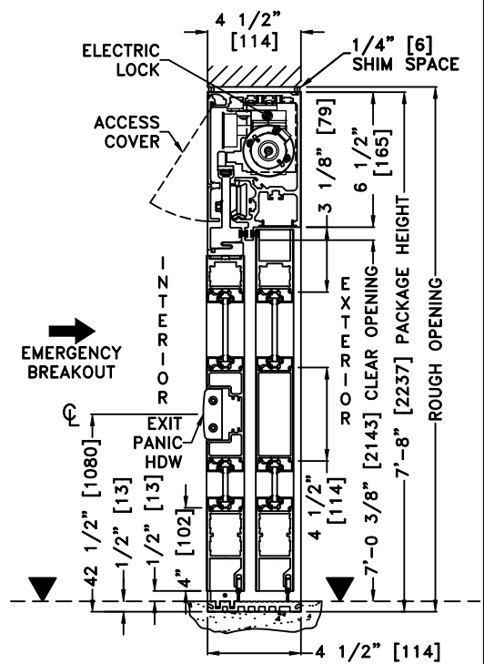
1 VERTICAL SECTION
