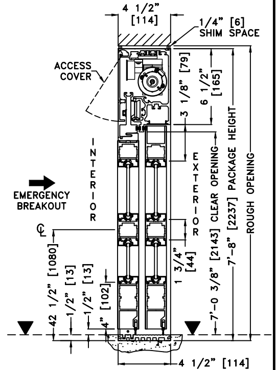
1 VERTICAL SECTION
