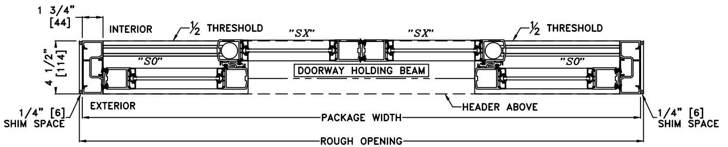
2 HORIZONTAL SECTION
