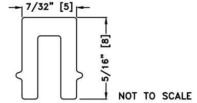
THRESHOLD TRACK GROOVE FILLER STRIP - RUNS THROUGH SLIDE DOOR OPENING ON ALL SLIDE DOOR TRACKS
