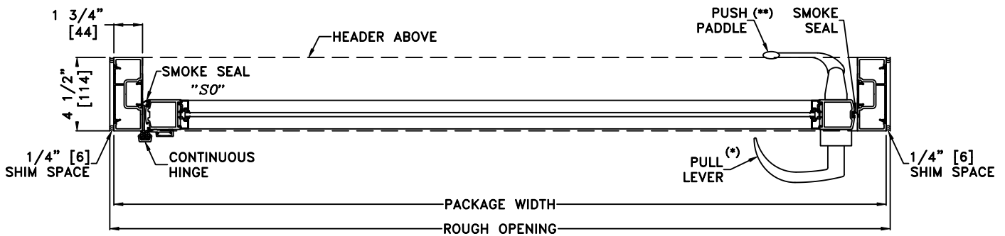
2 HORIZONTAL SECTION
