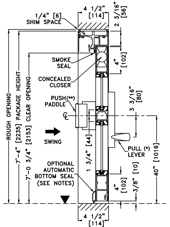
1 VERTICAL SECTION
