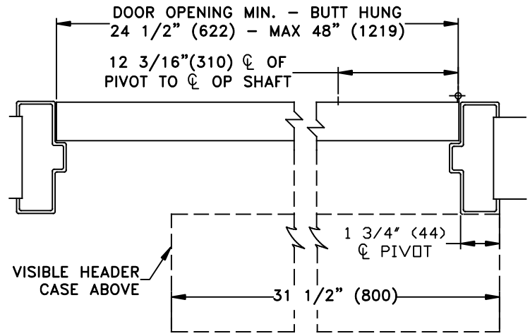
② HORIZONTAL SECTION
