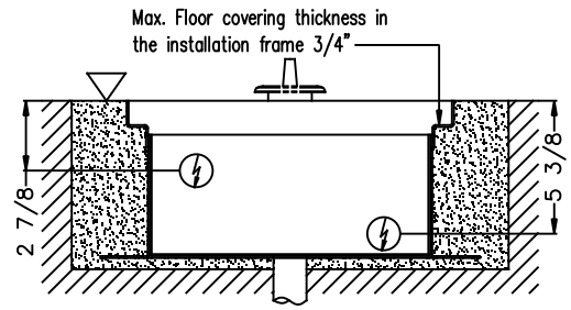
FLOOR BOX - OPTION B
