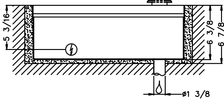
FRONT SECTION
