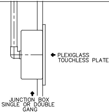
HARDWIRE – RECESS MOUNT
