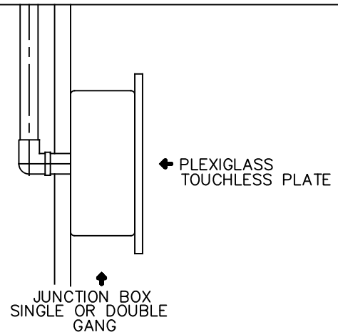
HARDWIRE – SURFACE MOUNT
