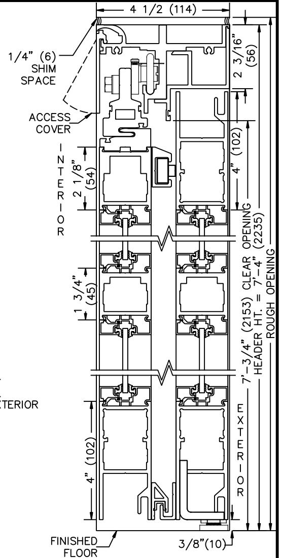
① VERTICAL SECTION
