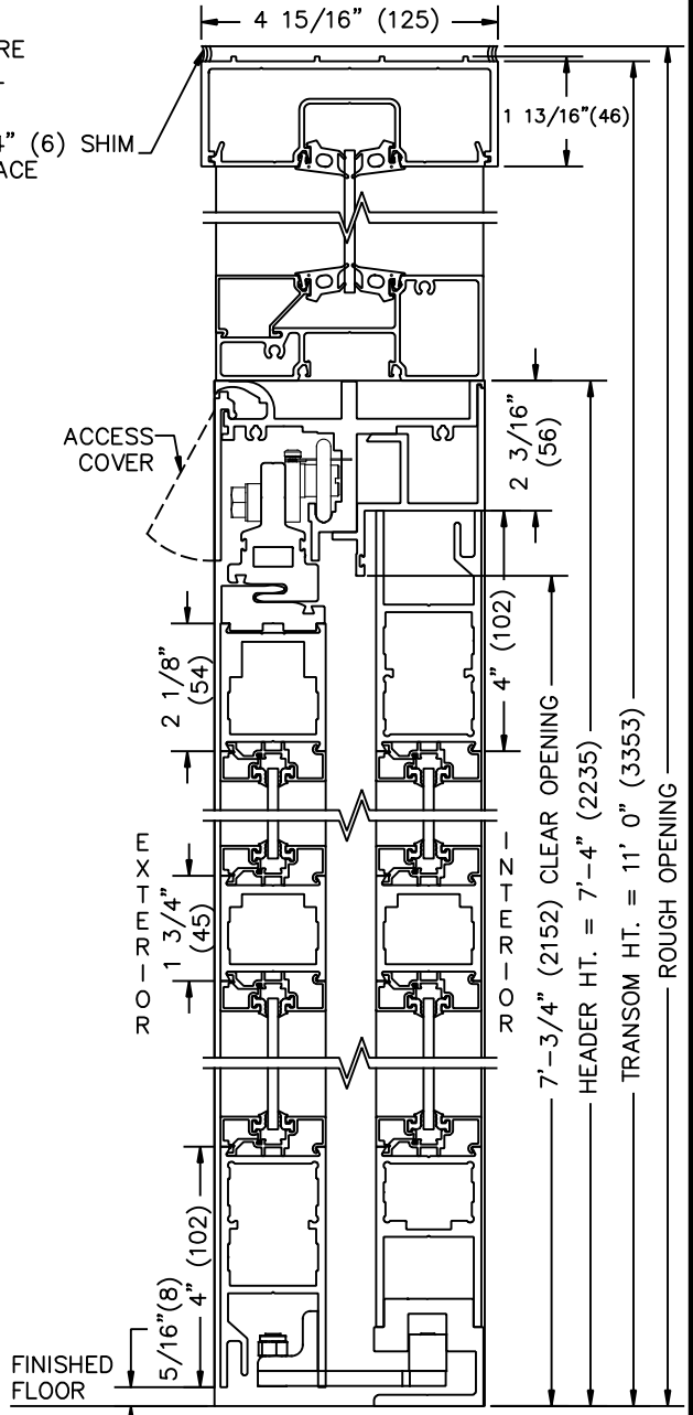
① VERTICAL SECTION
