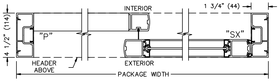
② HORIZONTAL SECTION
