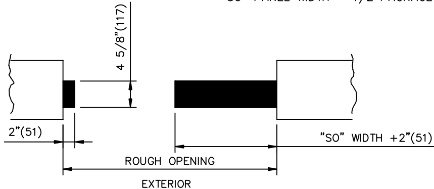
PLAN FOR BI-PART RECESSED THRESHOLD TRACK
