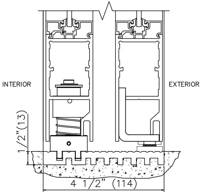
PLAN FOR SINGLE SLIDE RECESSED THRESHOLD TRACK
