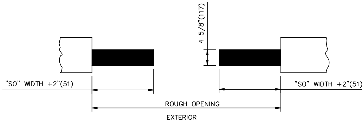
PLAN FOR BI-PART RECESSED THRESHOLD TRACK
