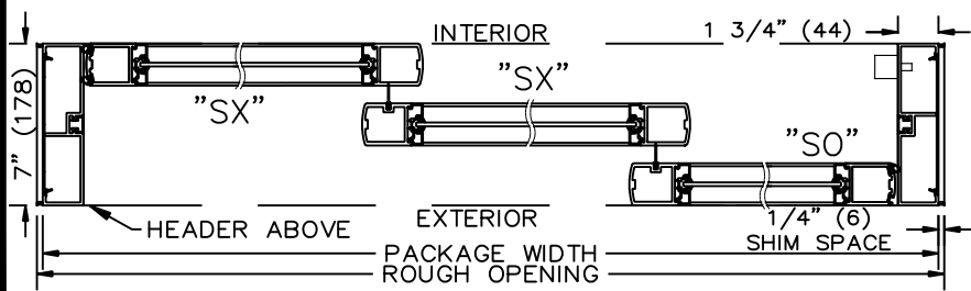
② HORIZONTAL SECTION
