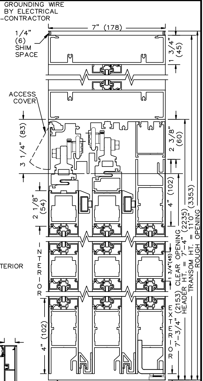
VERTICAL SECTION
