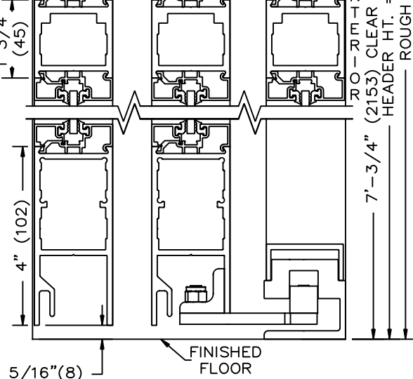
① VERTICAL SECTION
