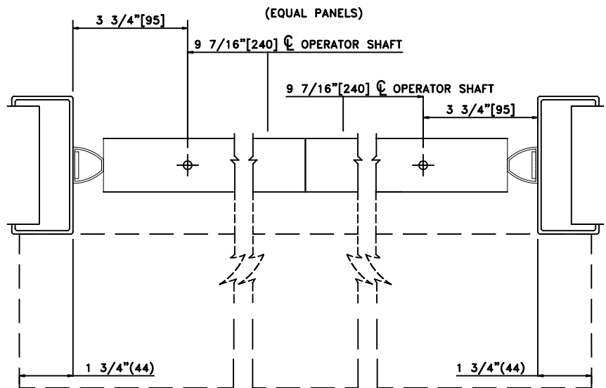
② HORIZONTAL SECTION
