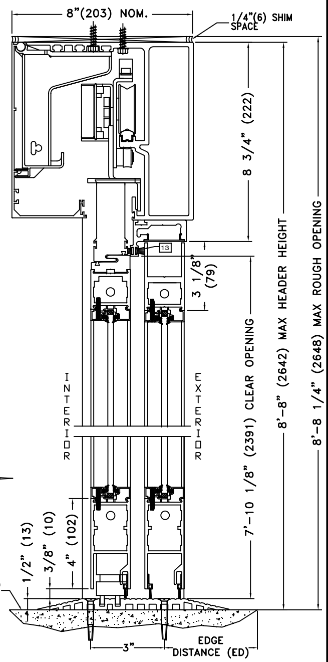
1 VERTICAL SECTION
